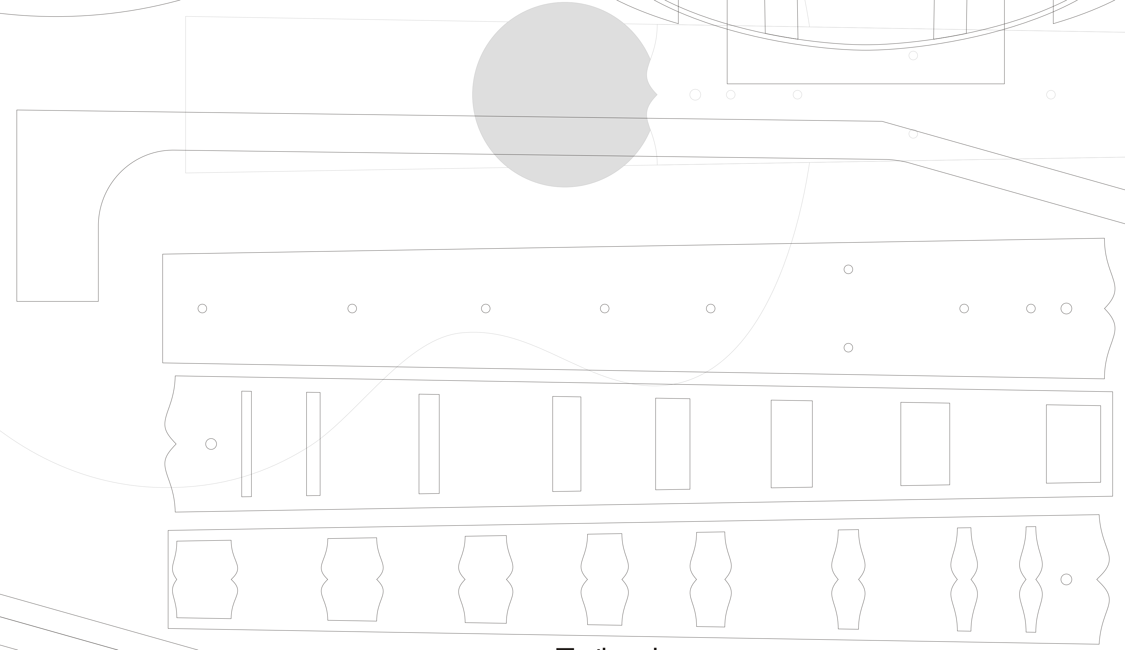
Fretboards
