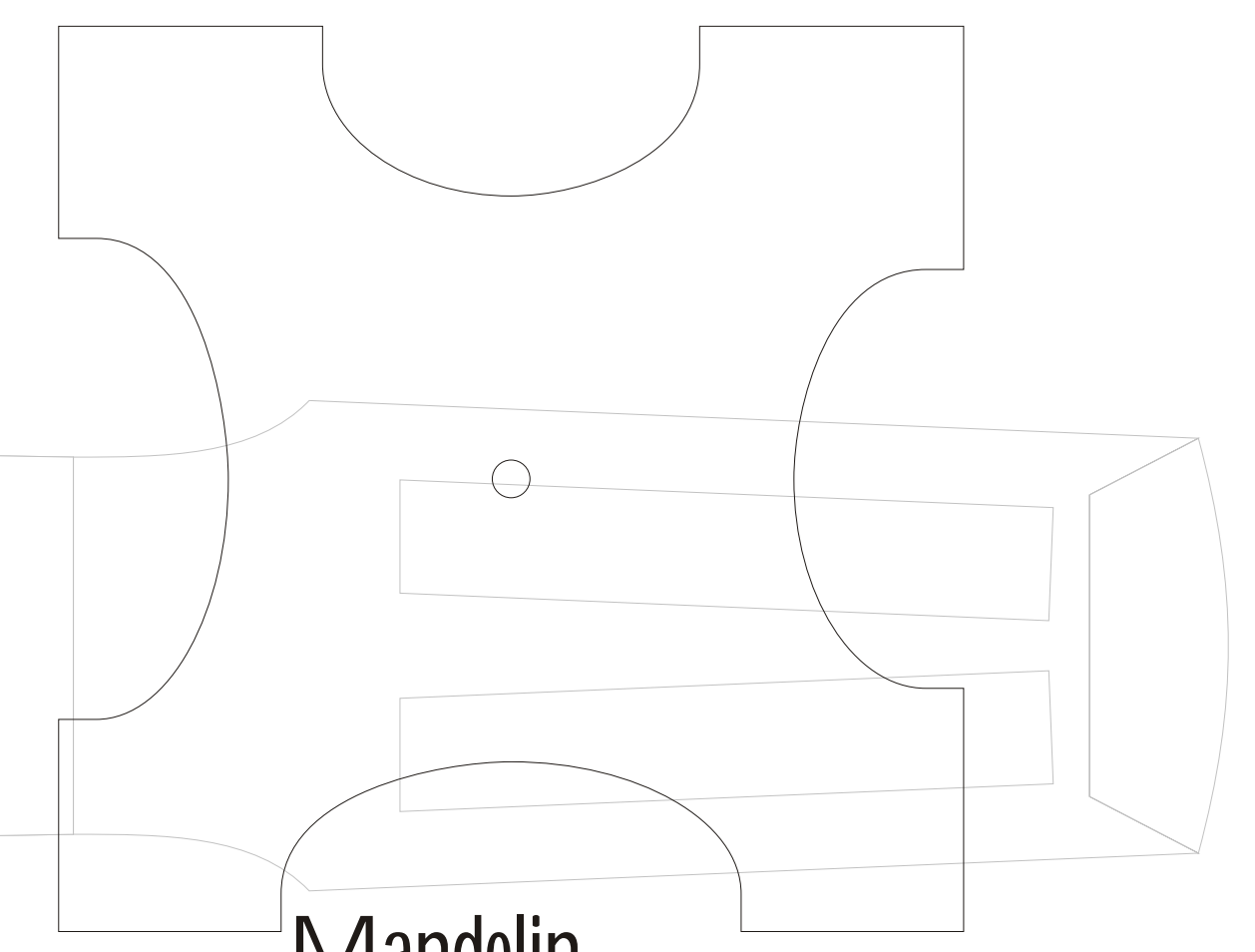
Mandolin nut, 5th, 12th 17th (25mm depth)
